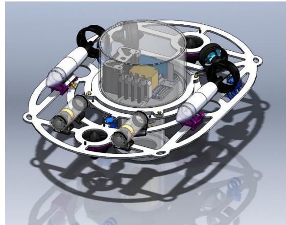
Figure 2: SolidWorks rendering of the AUV Poseidon
